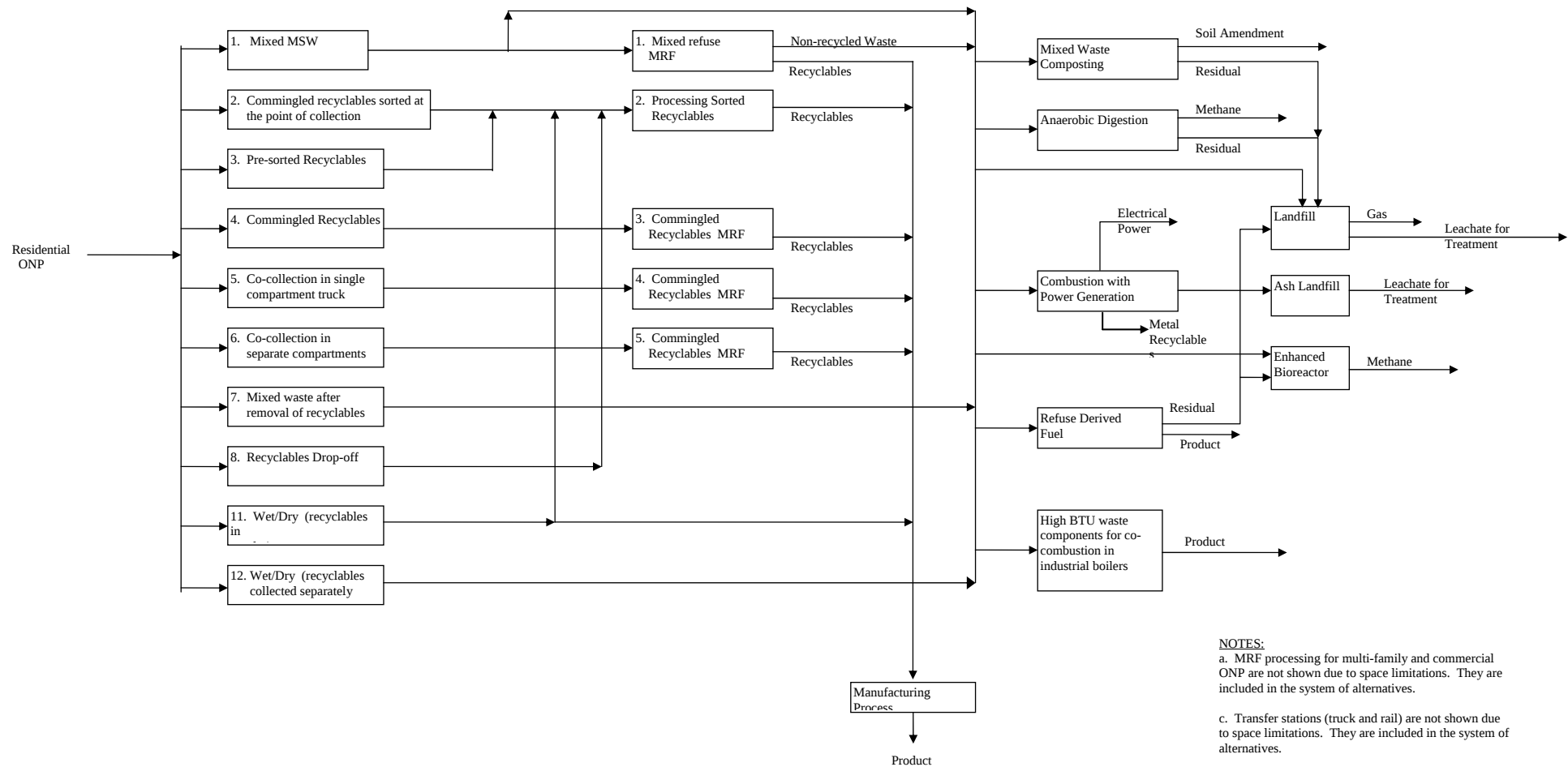
Figure 32. Waste Flow Alternatives for Residential Newspaper
