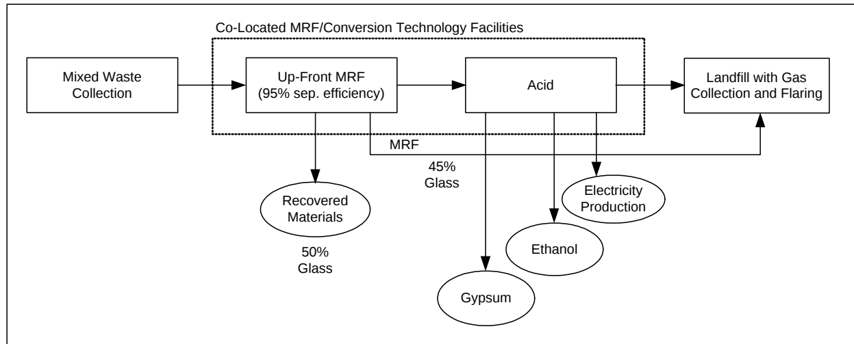
Figure 14. Acid Hydrolysis Scenario Design (Included as part of the conversion technologies scenario, Scenario 9.)
