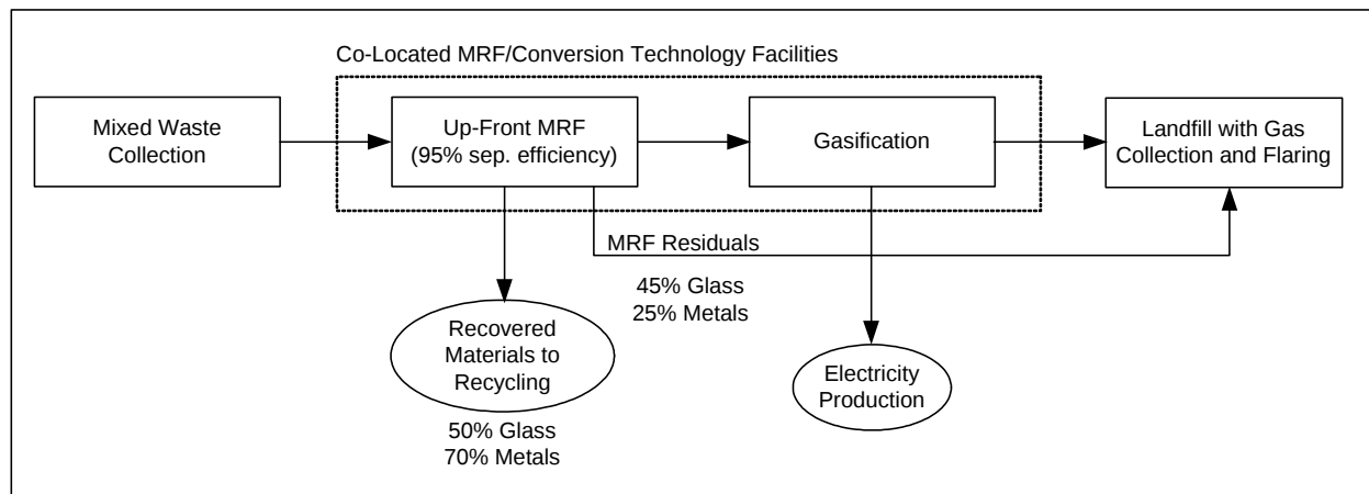
Figure 15. Gasification Scenario Design (included as part of the conversion technologies scenario, Scenario 9.)
