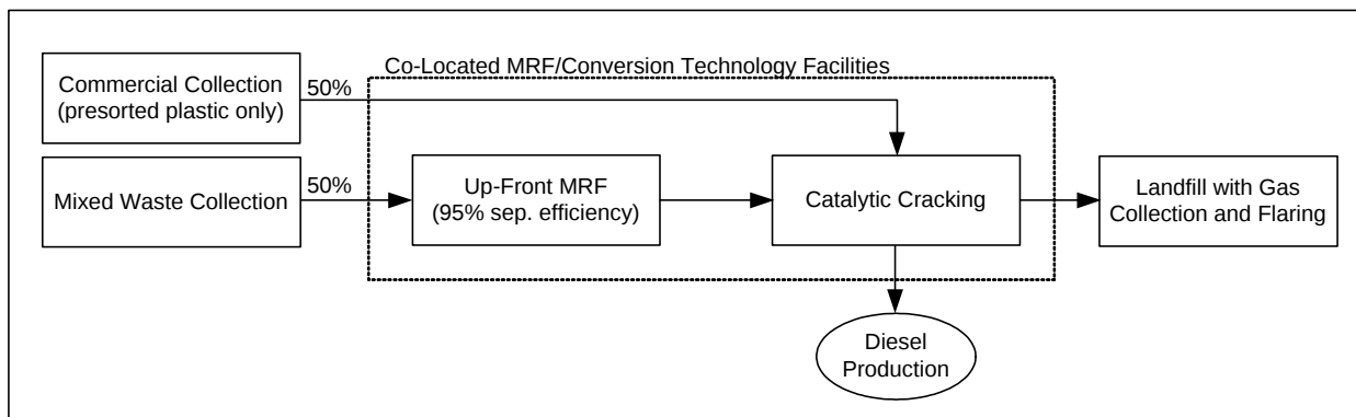
Figure 16. Catalytic Cracking Scenario Design (included as part of the conversion technologies scenario, Scenario 9.)
