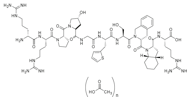
Figure 1 Chemical Structure
